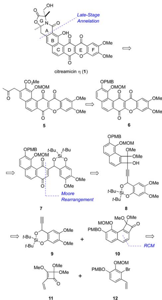
Scheme 1. Retrosynthetic Analysis of Citreamicin \eta
