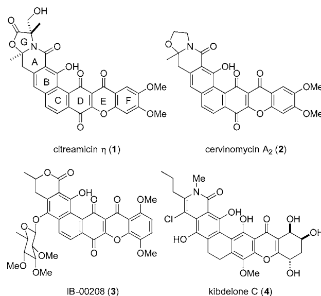
Figure 1. Polycyclic xanthone natural products.
